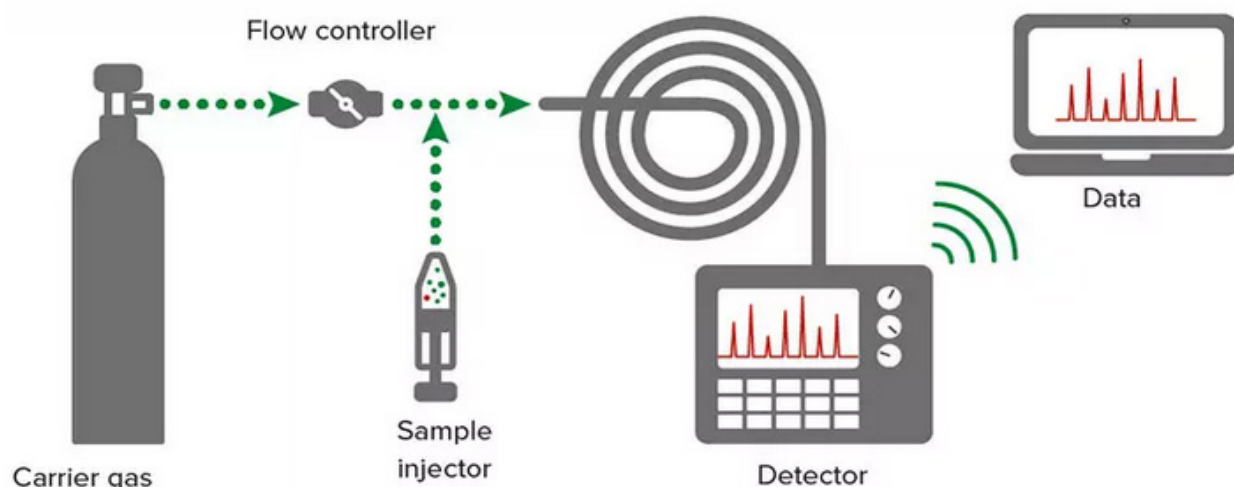
Figure 23: Illustration of the gas chromatography (GC) technique
