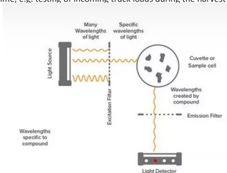
Figure 13: Schematic illustration of fluorometry where a sample is scattered with UV light and the emitted wavelength – specific to the sample - is measured
