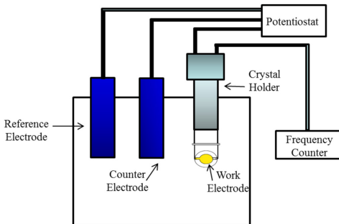
Figure 17: Schematic illustration of an electrochemical quartz crystal microbalance (EQCM) apparatus Source: Marrazza, 2014
