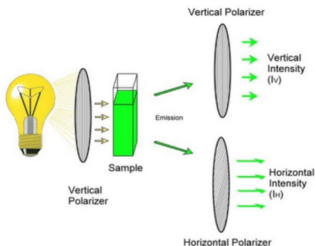
Figure 11: Schematic illustration of measurement of fluorescence polarization. Source: Maragos, 2009
