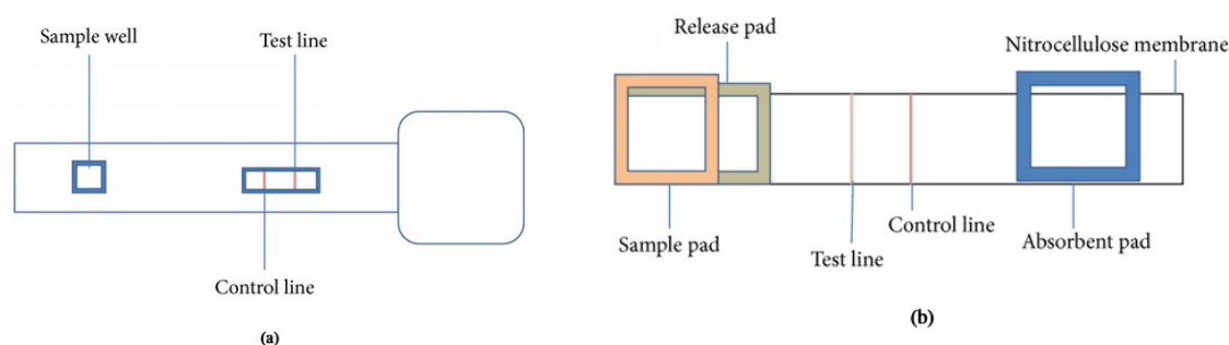
Figure 14: Schematic illustration of a lateral flow device in the dipstick format: (a) External details and (b) Internal details.
