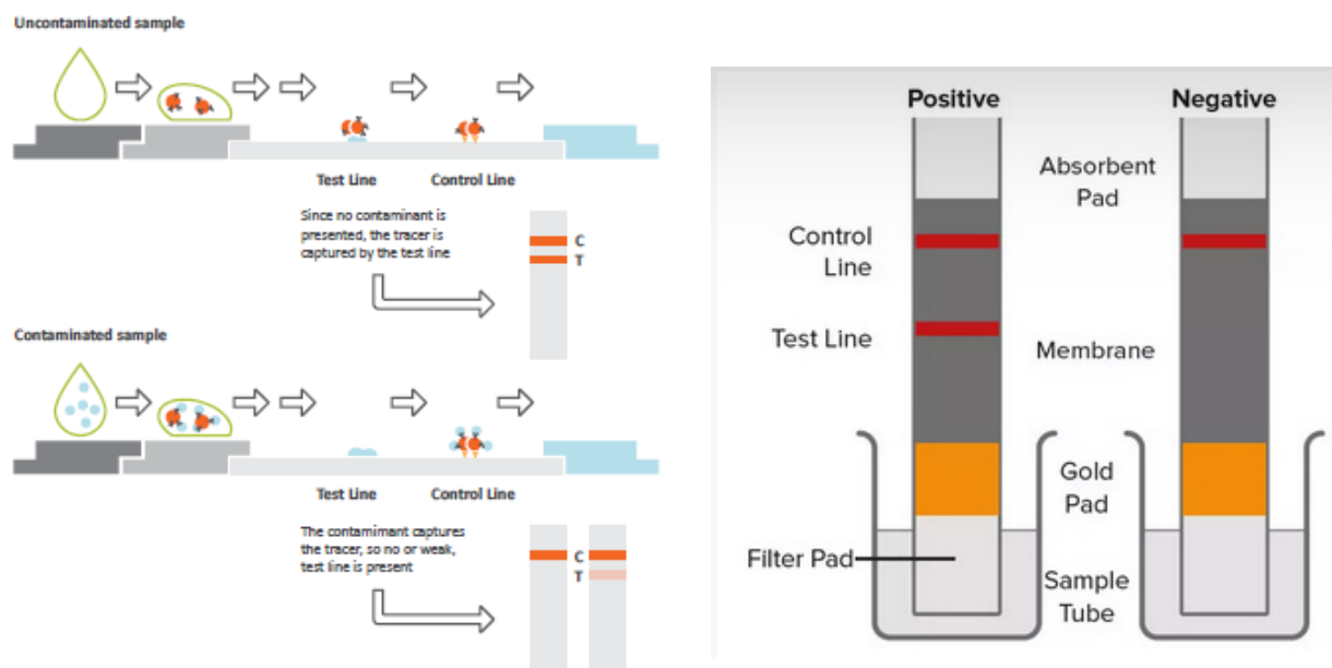
Figure 15: Illustration of a conventional lateral flow detection dipstick
