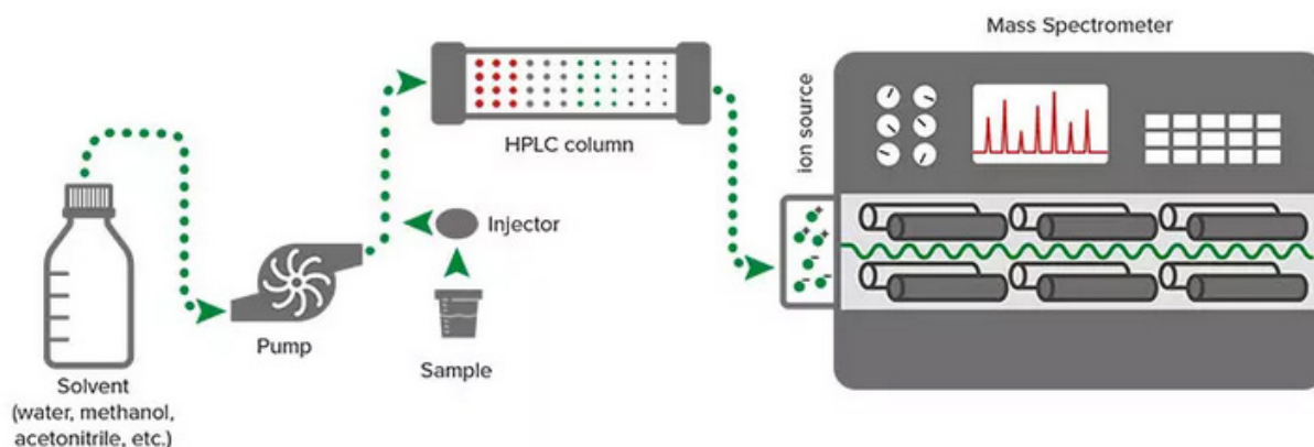
Figure 22: Illustration of the Liquid Chromatography-Tandem Mass Spectrometry (LC-MS/MS) technique
