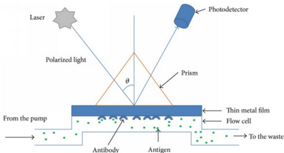
Figure 18: Surface plasmon resonance spectroscopy commonly used for the detection of antigen-antibody interactions in a buffered sample
